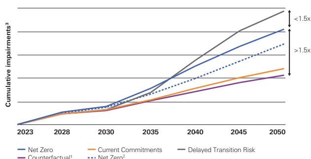
How credit losses from climate risks have been modelled under different transition scenarios
